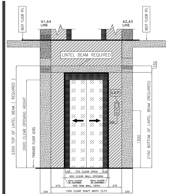
Sample Plan for custom shaft size
